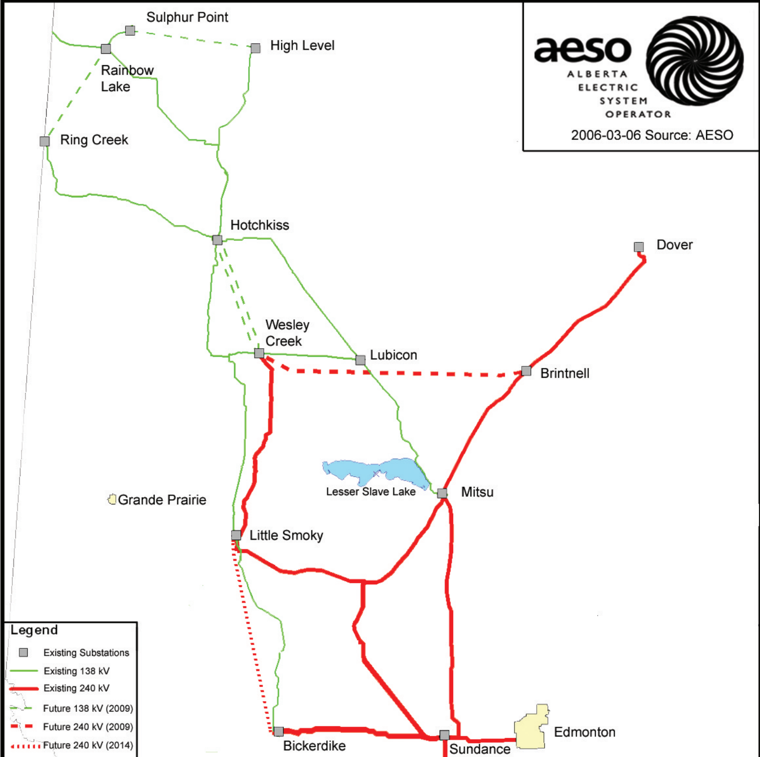
This diagram is a simplified version of the proposed and existing transmission system in the Northwest area of Alberta.
