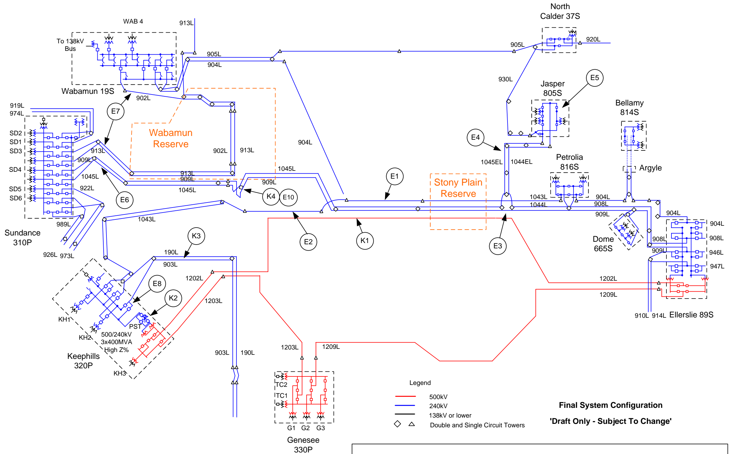
Keephills 3 and Edmonton Region 240 kV Line Upgrades Projects Final Configuration Based on Construction Plan of Aug 26, 2009 Page 2 of 6
