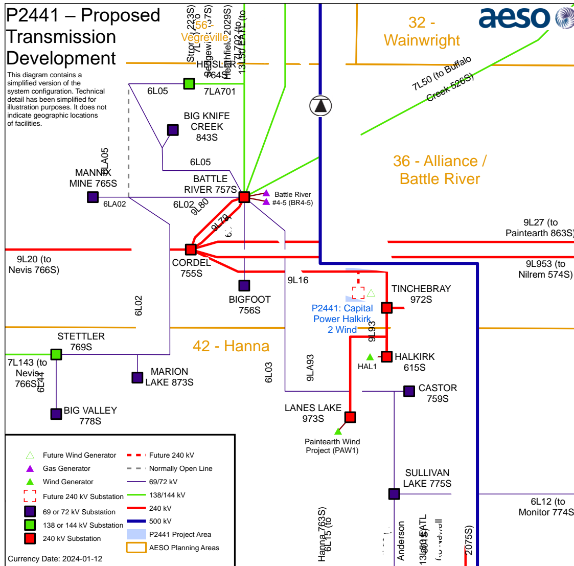
Figure 2-1: Proposed Transmission Development
