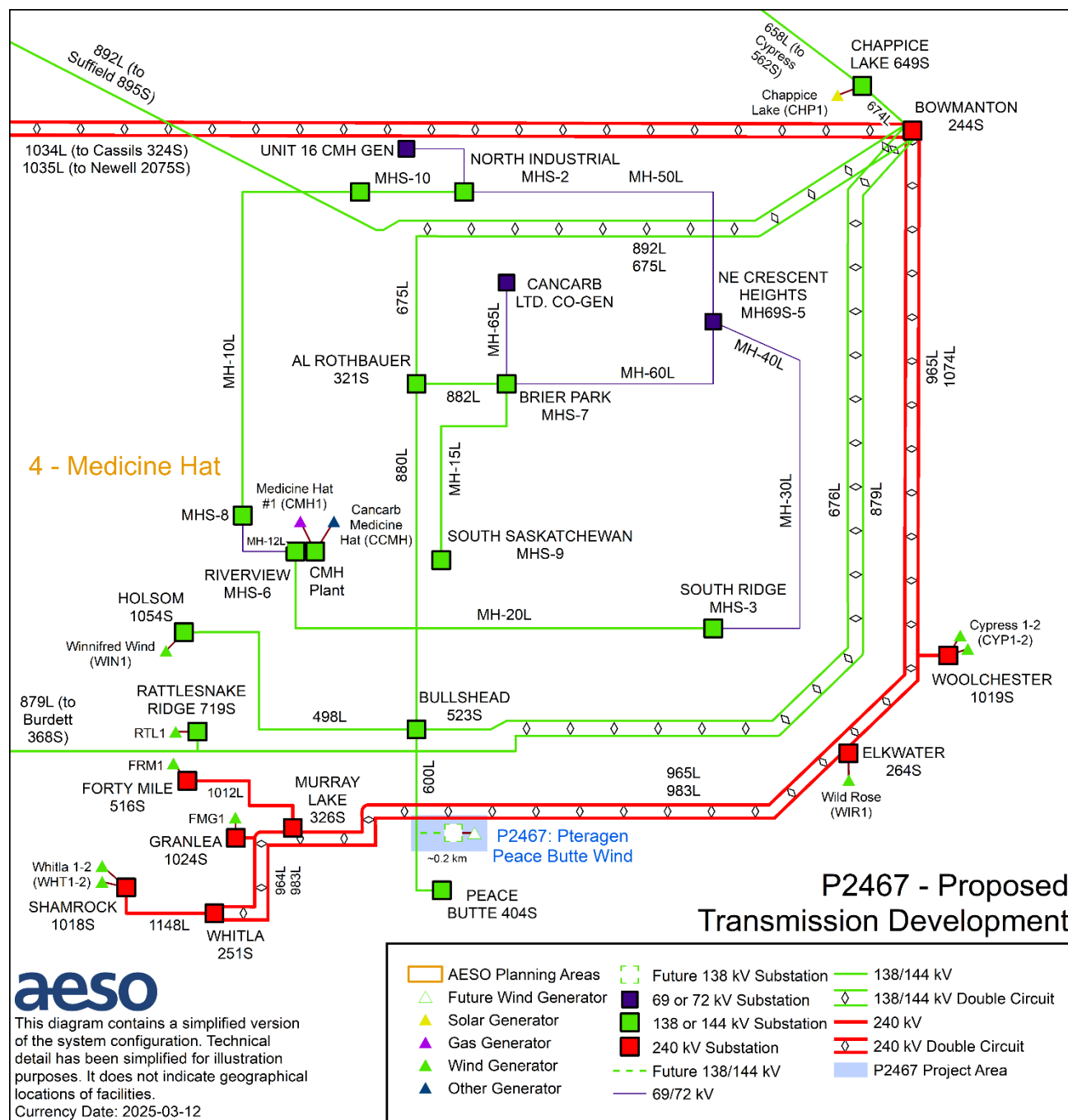
Figure 2-1: Proposed Transmission Development
