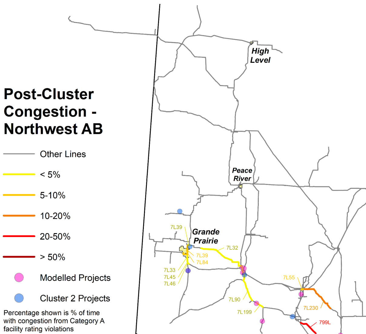
Figure 6 – Post-Cluster Congestion Frequency Heatmap
