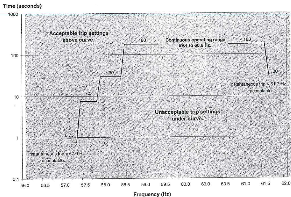
Figure 3-2: Generator Frequency Trip Setting
