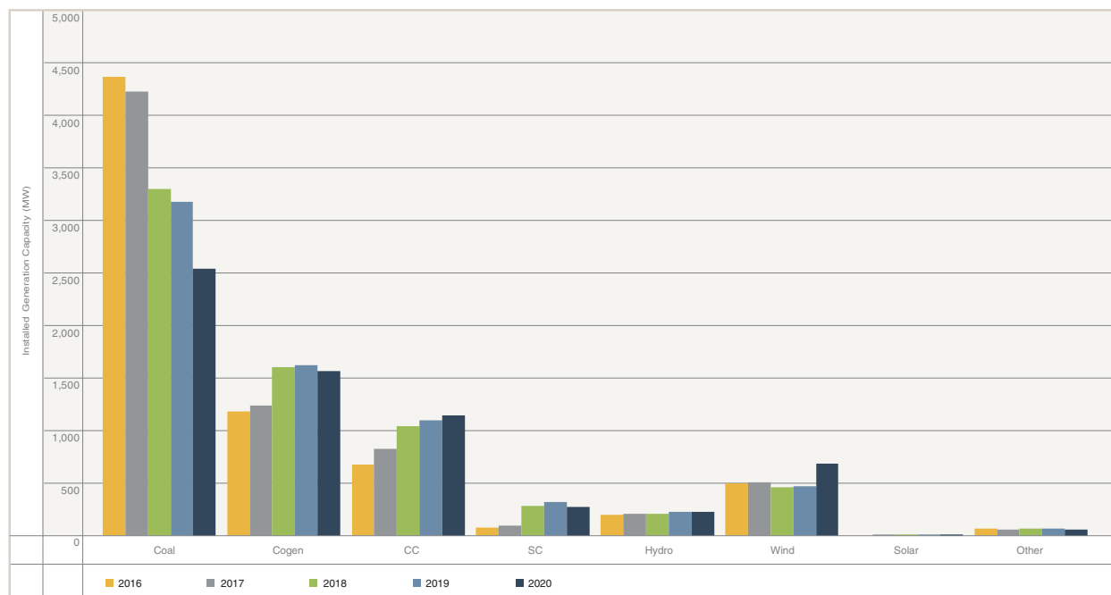
FIGURE 16: Annual average net-to-grid generation by technology
