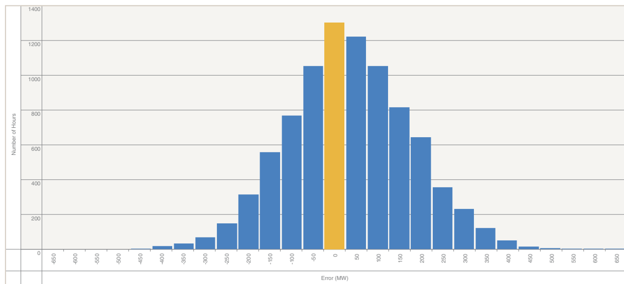
FIGURE 40: Distribution of day-ahead load forecast error in 2020
