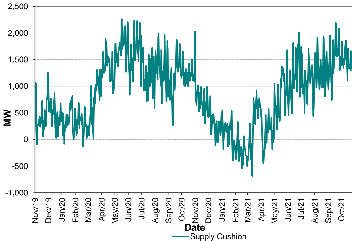
Figure 2: Alberta Interconnected Electric System (AIES) Daily Supply Cushion, November 1, 2019 to October 31, 2021
