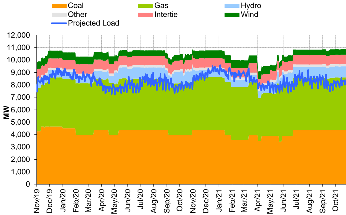
Figure 3: Alberta Interconnected Electric System (AIES) Daily Peak Demand and Available Supply, November 1, 2019 to October 31, 2021
