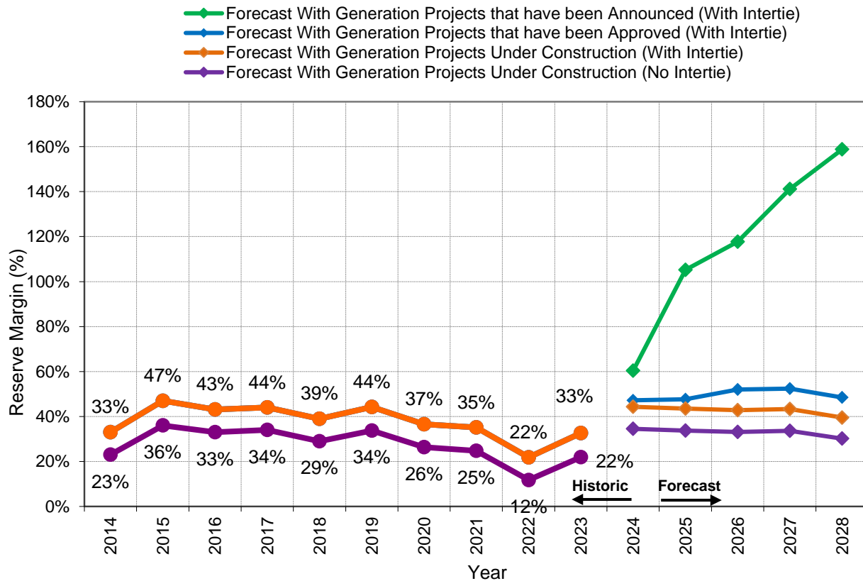
Figure 1: Alberta Interconnected Electric System (AIES) Reserve Margin, 2014 – 2028
