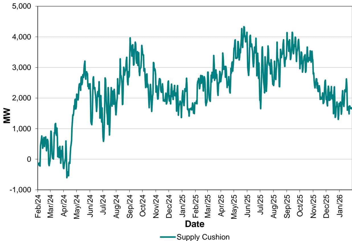
Figure 2: Alberta Internal Load (AIL) Daily Supply Cushion, Feb 1, 2024, to Jan 31, 2026
