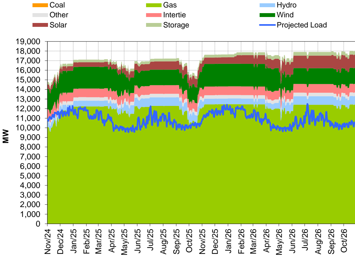
Figure 3: Alberta Internal Load (AIL) Daily Peak Demand and Available Supply November 1, 2024, to October 31, 2026
