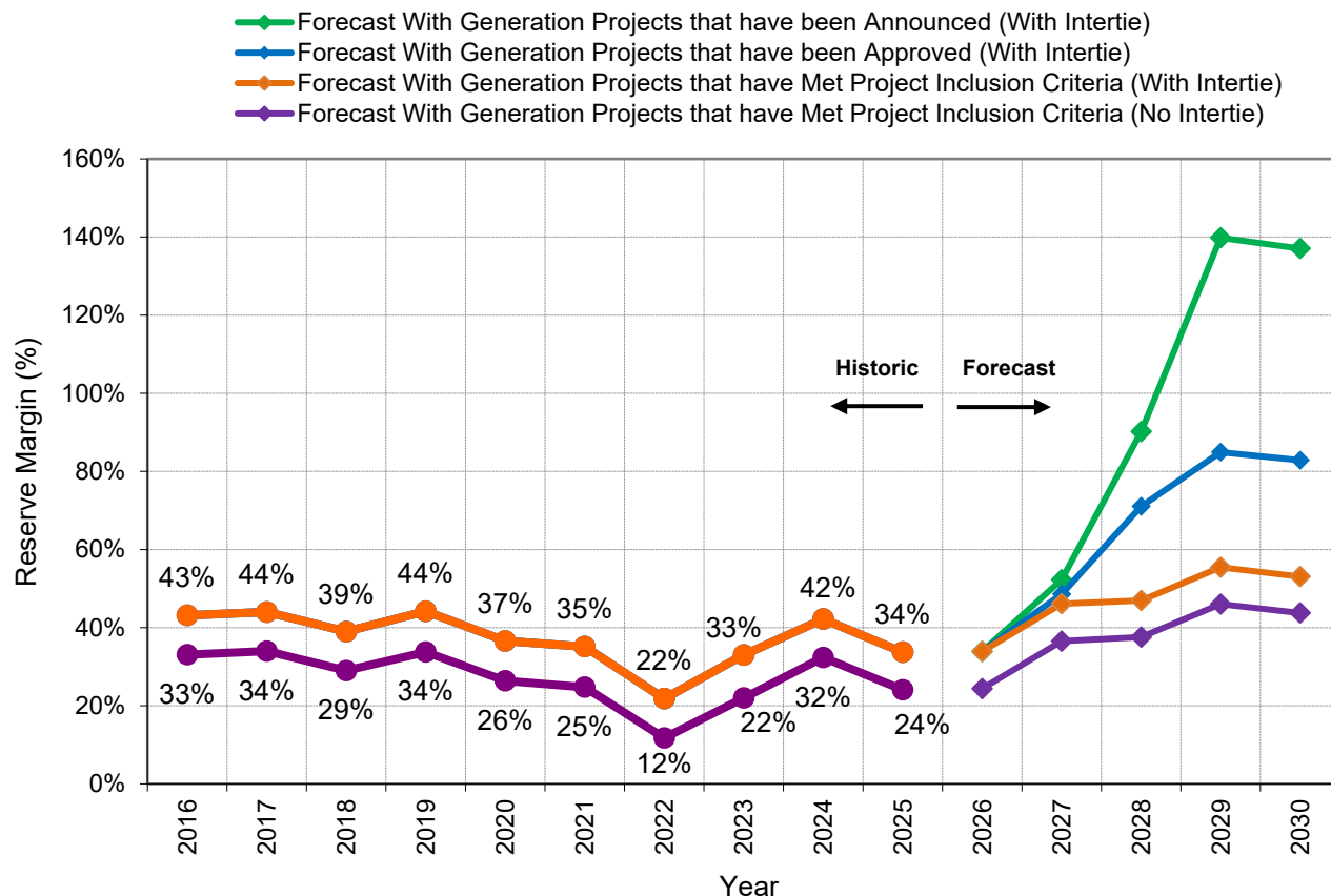
Figure 1: Alberta Interconnected Electric System (AIES) Reserve Margin, 2016 – 2030
