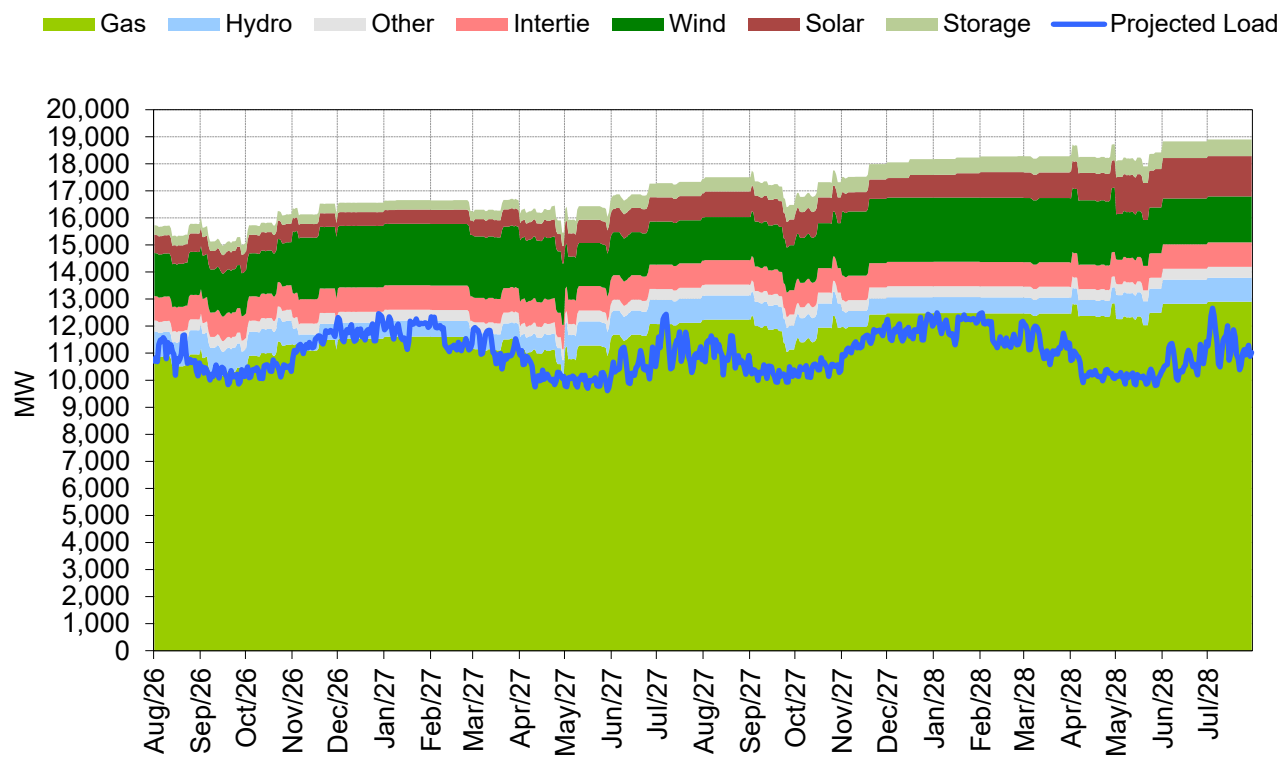
Figure 3: Alberta Internal Load (AIL) Daily Peak Demand and Available Supply August 1, 2026, to July 31, 2028
